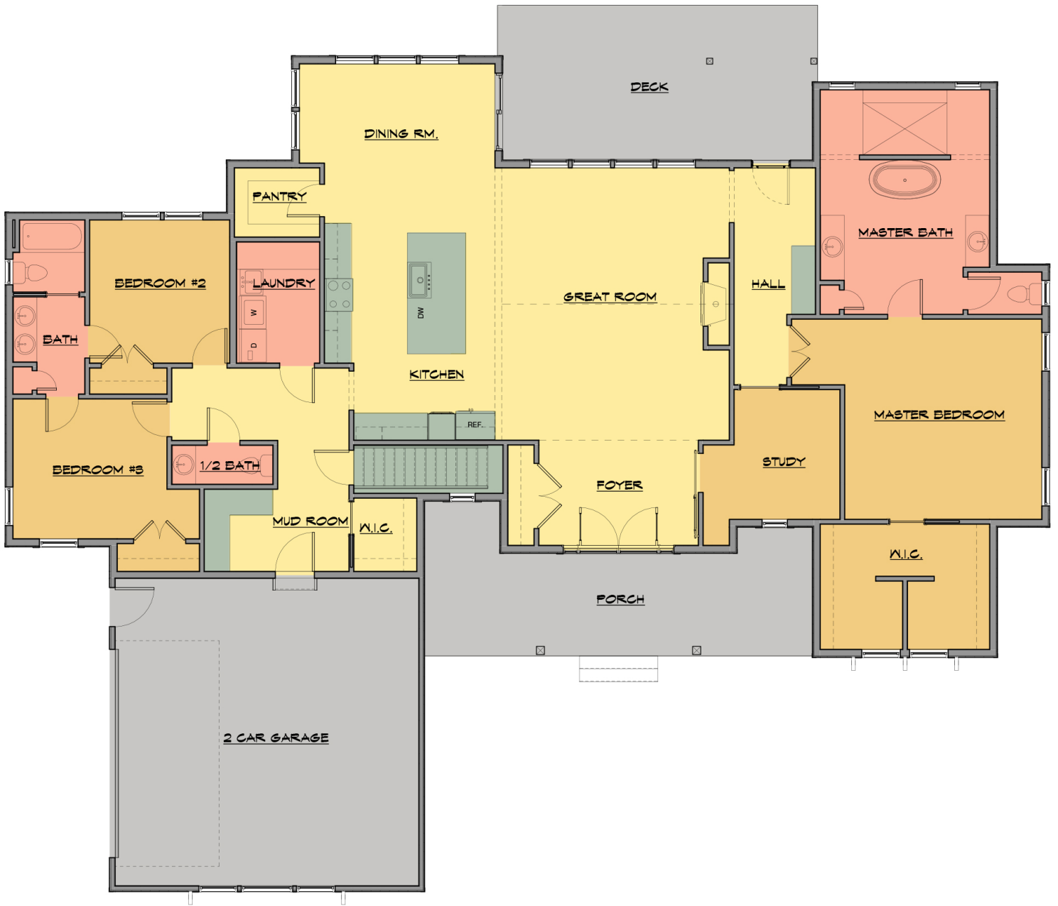
First Floor Plan Square Footage - 2,624sq.ft.
